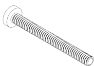
4x M4x35 screw with cross slot ( SP33 )
